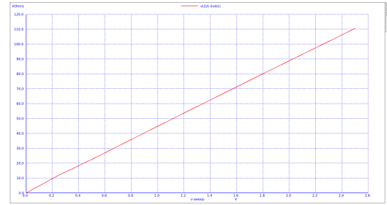
(b) Absolute resistance of nmos transistor and V_{gs} = 1.2V
